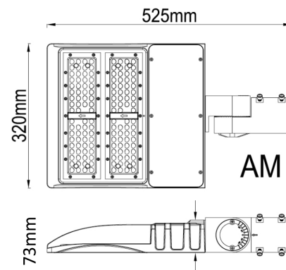
DIRECT MOUNTING
